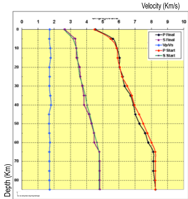
FIG. 6. Starting and final (bold) 1D P- and S-wave models with corresponding Vp/Vs ratio for S out-eastern Albania. The P-velocity gradient decreases at the Moho and in the upper mantle (Zone 3).
