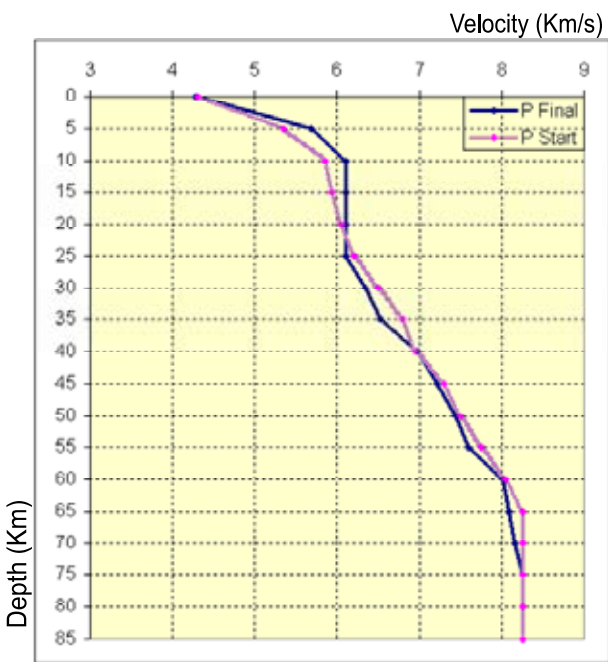
FIG. 5. Starting and final (bold) 1D P- or S-wave model for Southwestern Albania. The P-velocity gradient increases in upper and middle crust and decreases in the lower crust and upper mantle (Zone 2).
