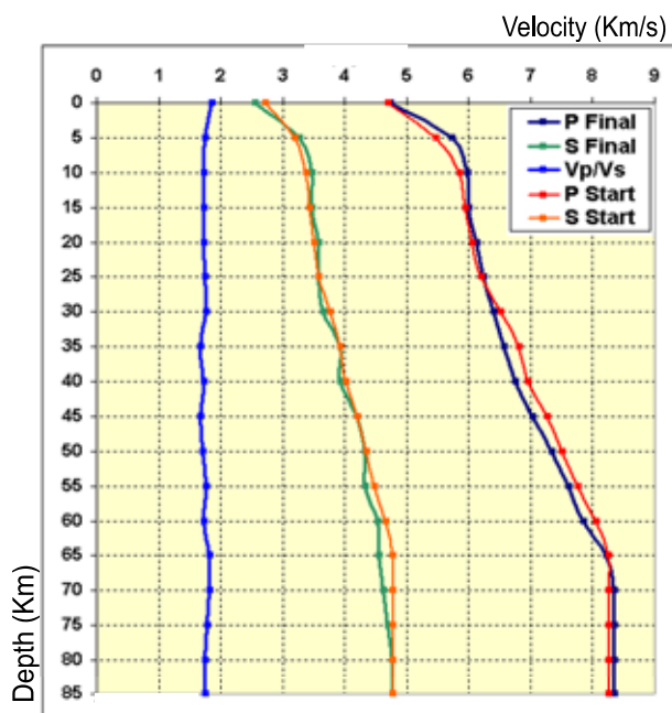
FIG. 8. Starting and final (bold) 1D P- and S-wave models with corresponding Vp/Vs ratio for Northern Albania. The P-velocity gradient increases in upper and middle crust and decreases in the lower crust (Zone 5).
